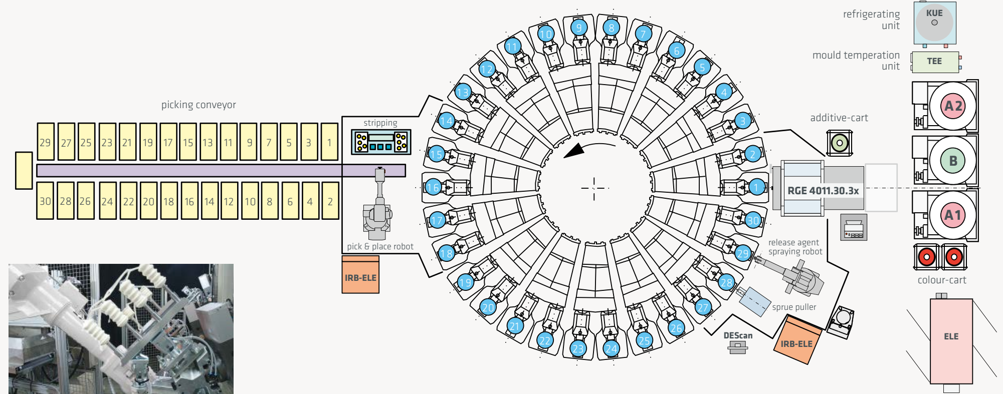
PICK & PLACE
