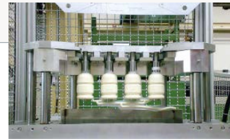
STRIPPING
