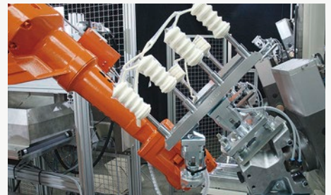
HANDLING-ROBOTER
